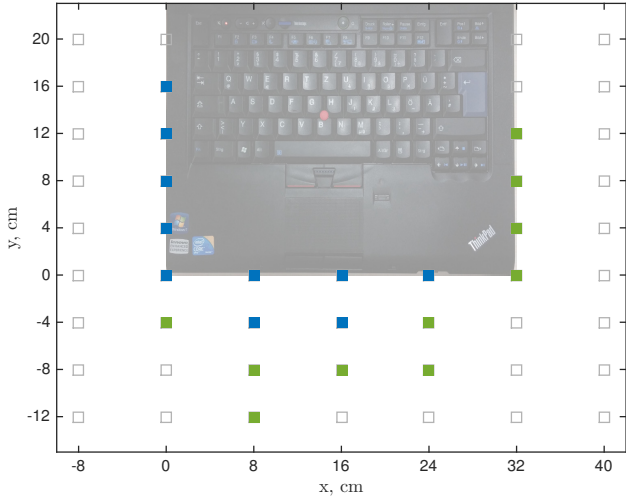
Fig. 6. Presence of the signal. Green marks show a successfully decoded signal using the periodic-based scheme. Blue indicate positions where both encoding schemes are feasible. White marks indicate no detectable signal. We use the following parameters: amplitude modulation: t_0 = 0.5s , bitrate 2bit/s; periodic-based modulation: t_0 = 0.25s , t = 15s , p_0 = 3 , p_1 = 5 , bitrate 0.067bit/s.
