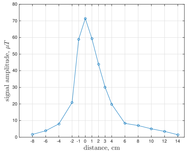
Fig. 5. Magnitude of the signal depending on the distance from the source B .
