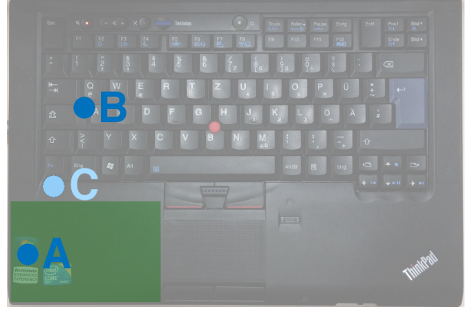
Fig. 1. The position of the hard drive (green), sources of EM signal A, B and intermediate point C.
