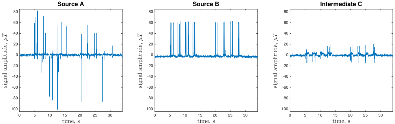
Fig. 2. Measured EM-fluctuations at points A , B and intermediate point C .
