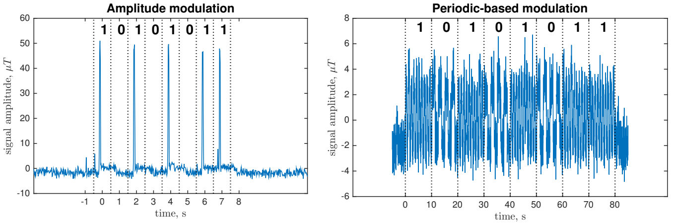
Fig. 4. Examples of two modulation schemes. Amplitude modulation: t_0 = 1s , bitrate is 1bit/s. Periodic-based modulation: t_0 = 0.25s , t = 10s , p_0 = 5 , p_1 = 3 , bitrate is 0.1bit/s.
