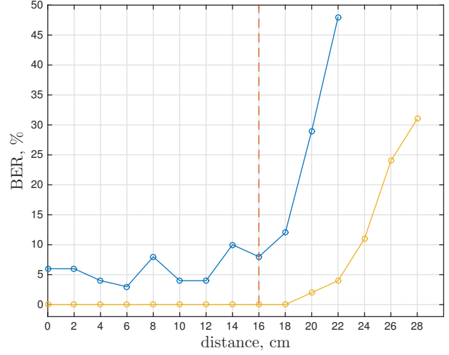
Fig. 7. BER depending on the distance from the point B. Area outside the laptop starts from 16cm. We use the following parameters: amplitude modulation (blue): t_0 = 0.5s , bitrate 2bit/s; periodic-based modulation (yellow): t_0 = 0.25s , t = 15s , p_0 = 3 , p_1 = 5 , bitrate 0.067bit/s.
